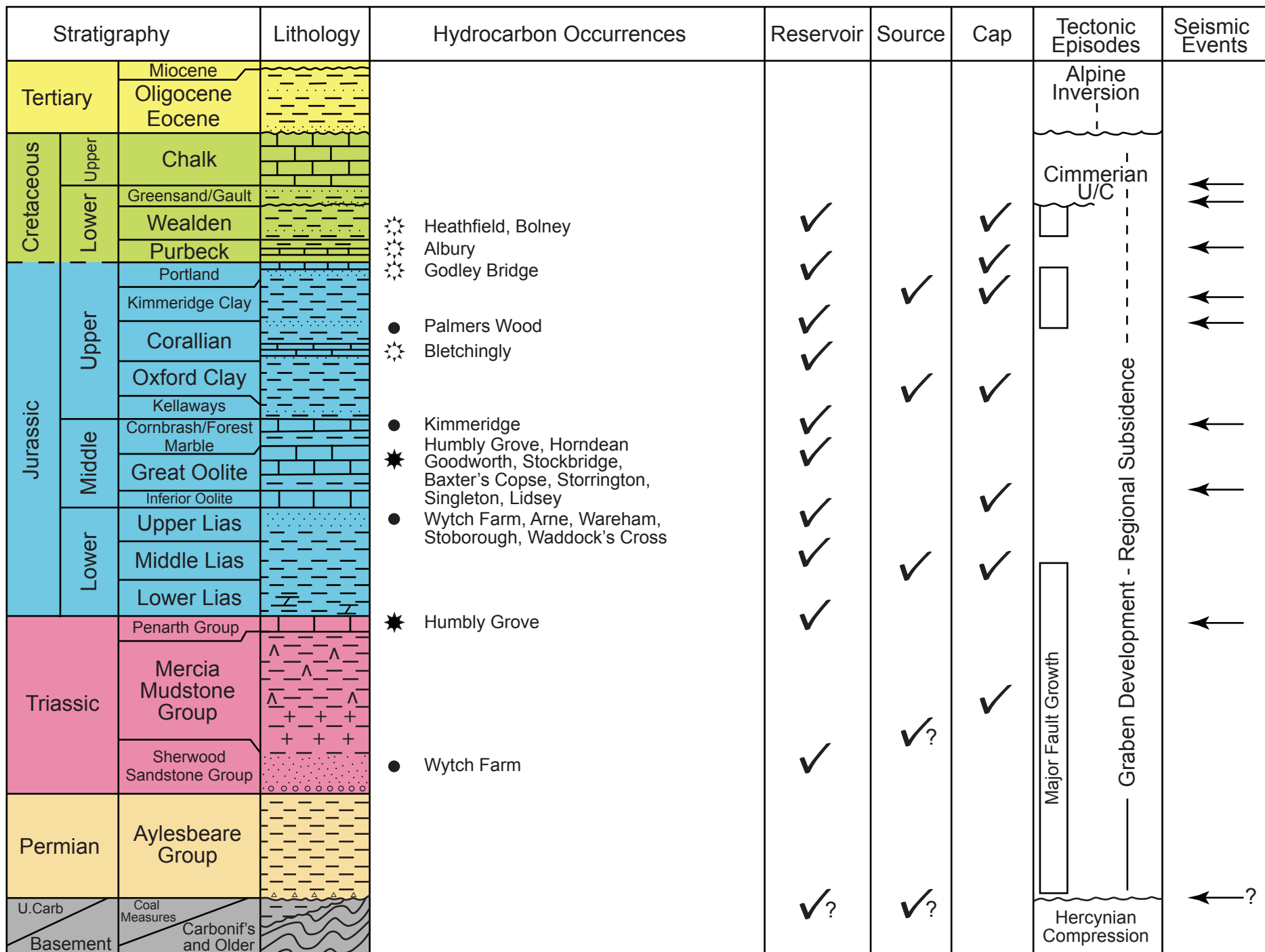
Fig. 2 Southern England stratigraphic column, showing hydrocarbon occurrences
